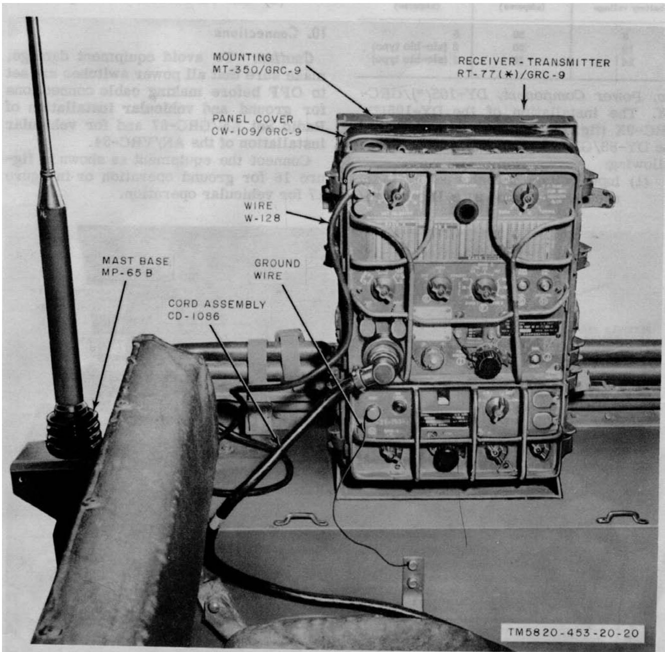
Figure 14. RT-77(*)/GRC-9, typical vehicular installation.
